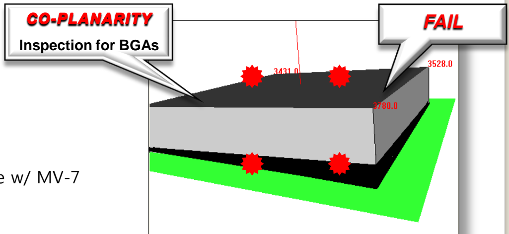
Actual Inspection Results for Lifted BGA
