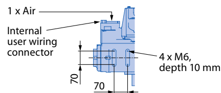
View D
