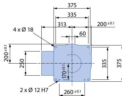
View C
